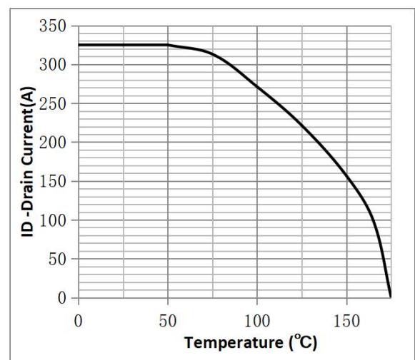
Fig.12 ID vs. Junction Temperature 2
